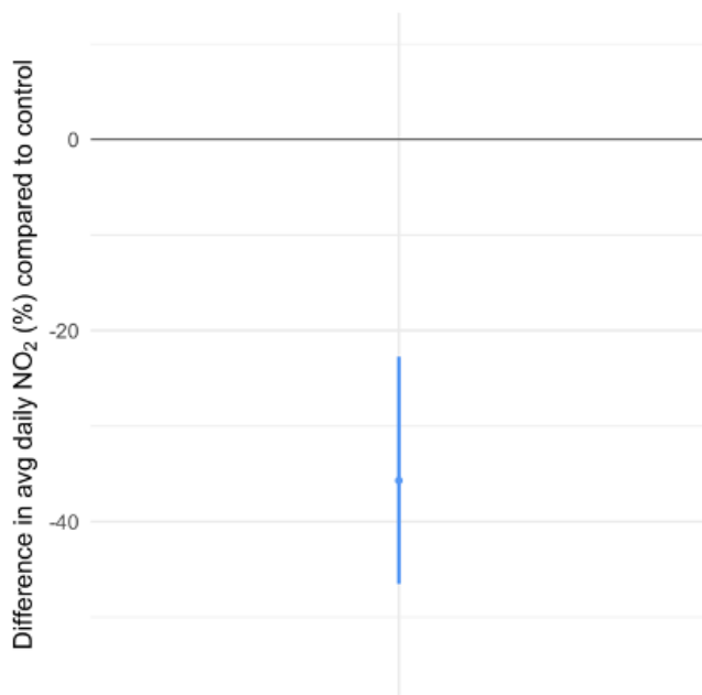
Figure B1. Effect of the induction stove intervention on daily average NO 2 exposure in a 24-hour period. Post intervention NO 2 levels were 35.7% lower (indicated with the dot) in kitchens with induction stoves compared to those with the gas stoves after adjusting for outdoor temperature, apartment level, and street orientation. 95% confidence intervals were -46.5 to -22.7% (indicated with the error bars).
