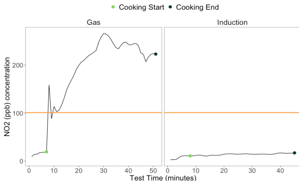
Figure 2: Real time NO 2 (ppb) concentrations during controlled cooking events with a gas and induction stove, respectively. The start of the cooking is noted with a light green dot and the end noted with the dark green dot. The orange horizontal line (101 ppb) indicates the EPA threshold for one-hour NO 2 averages that are considered “Unhealthy for Sensitive Groups.”
