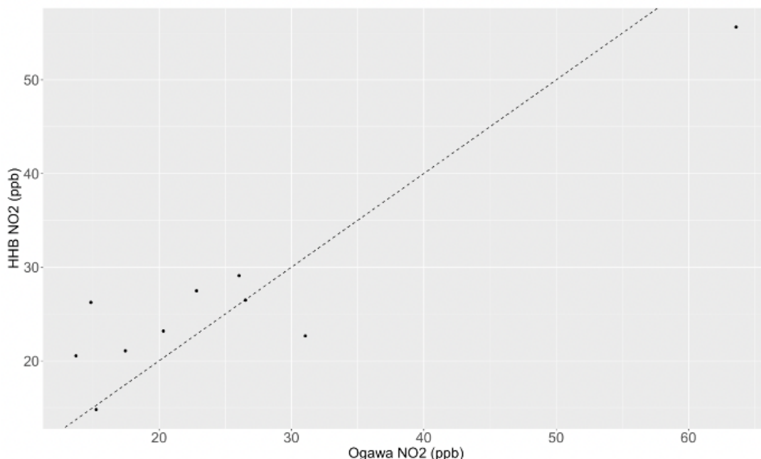
Figure A1. Relationship between the Home Health Box and Ogawa Badge NO 2 measurements
